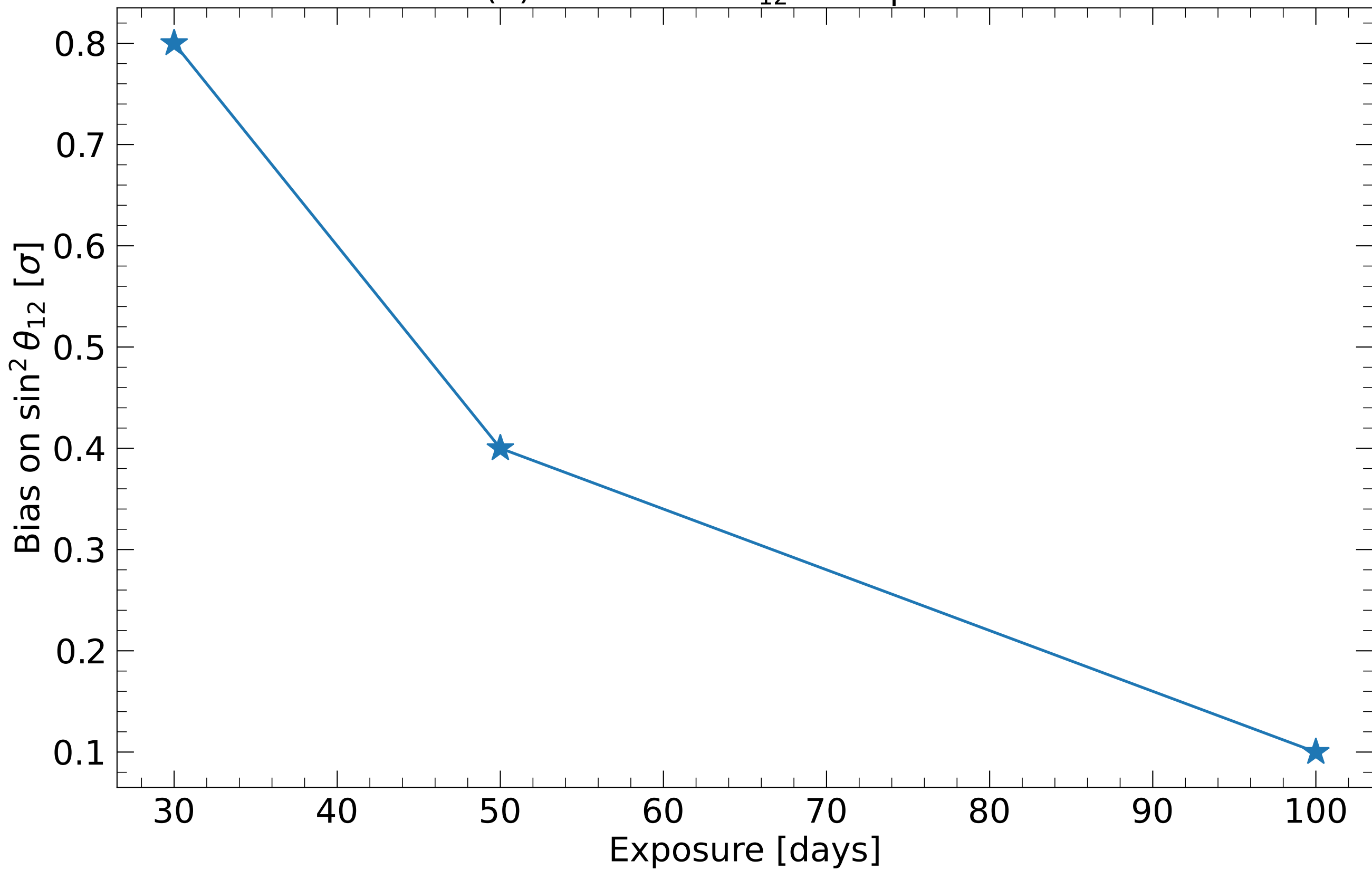
(b) Bias of \sin^2 \theta_{12} vs Exposure
